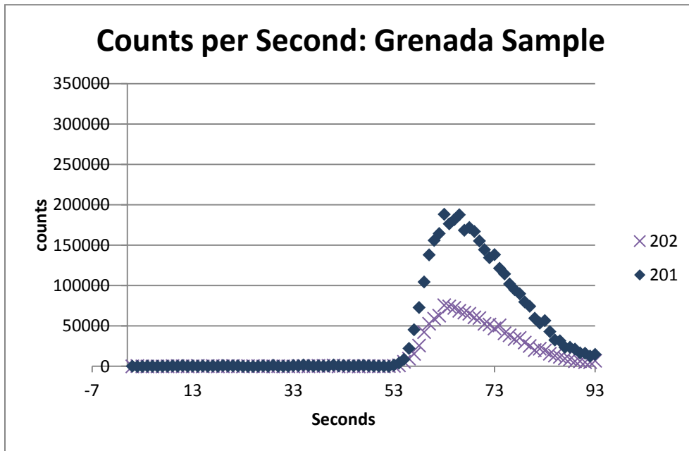
Figure 8: Counts/Second of Grenada Sample shows that there is more ^{201}\text{Hg} than ^{202}\text{Hg} .
