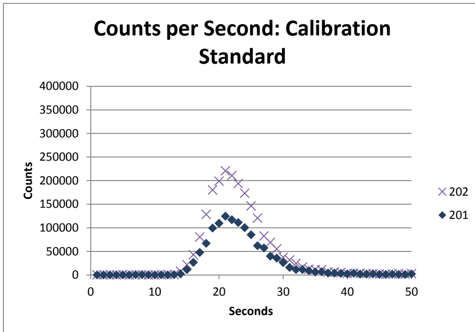
Figure 9: Counts/Second of the calibration standard shows that there is more ^{202}\text{Hg} than ^{201}\text{Hg} , which agrees with the natural occurrence of mercury isotopes.
